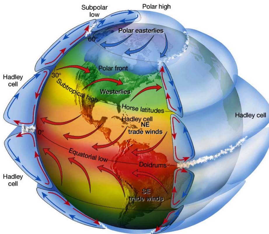
FIGURE 2-1. Hadley Cells.
