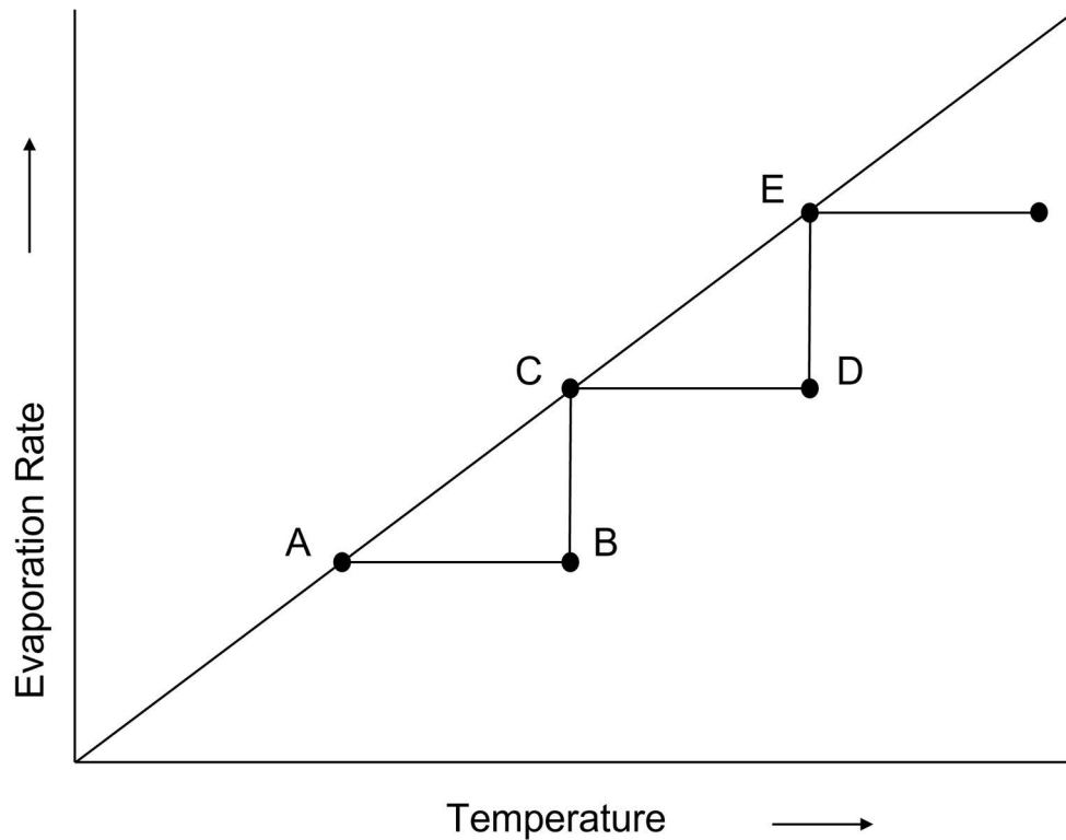
FIGURE 2-11. Positive feedback.
