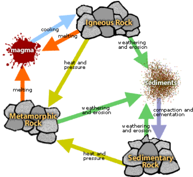
FIGURE 2-6. Rock cycle.
