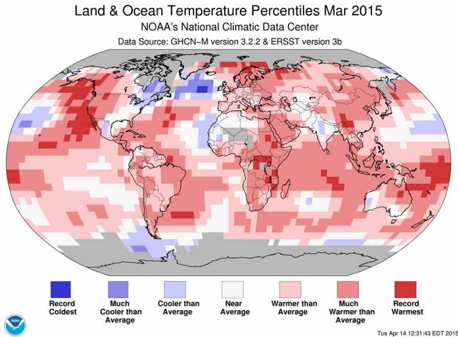
FIGURE 5-4. NOAA Monthly Temperature Change
